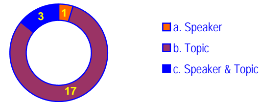
Event Selection
